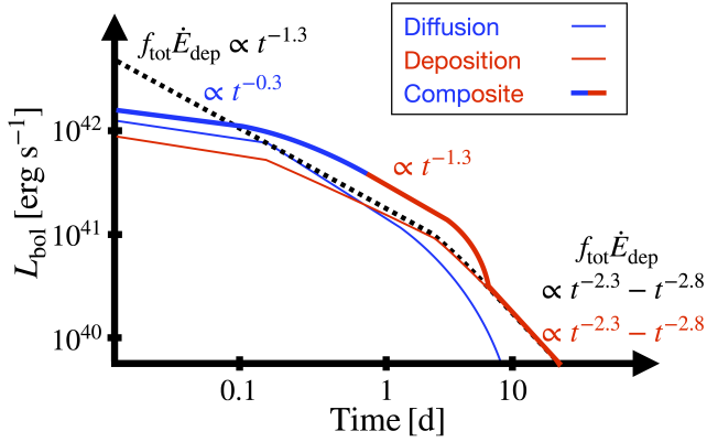
Figure 1. Time evolution of r-process powered KN light curve. The early blue KN emission (thick blue line) is \propto t^{-0.3} as it is mostly powered by diffusion emission (thin blue line) [first term in equation (5)]. After a transitional phase, later emission (thick red line) follows deposition rate of thermal energy through r-process (thin red line in the optically thin part; and dashed line in the whole ejecta) as \propto t^{-1.3} [second term in equation (5)], and asymptotically \propto t^{-2.3} - t^{-2.8} (for a similar figure see Figure 4 in Kasen & Barnes 2019; also see Waxman et al. 2019; Hotokezaka & Nakar 2020).
