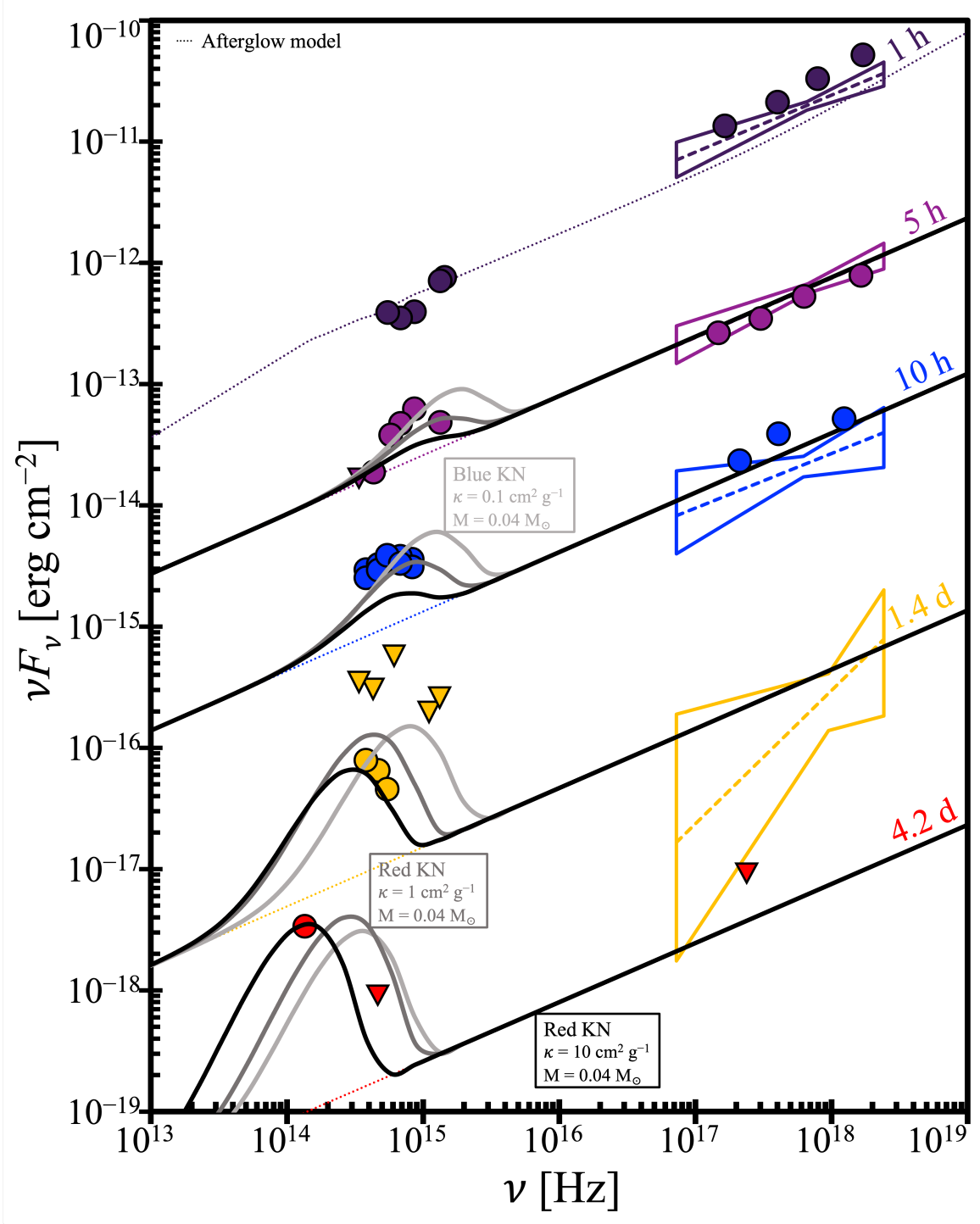
Figure 3. SED of GRB 211211A and its time evolution. Five epochs are shown: 1 h (dark purple), 5 h (purple), 10 h (blue), 1.4 d (orange), and 4.2 d (red). Filled circles indicate detections, while triangles indicate upper limits. Central values for the X-ray’s photon index (dashed lines) and the corresponding uncertainty (bow ties) are shown (see Section A). The afterglow model is shown at each epoch with a dotted line. Three r-process KN models are shown (using z = 0.0762 ): A low opacity blue KN model ( \kappa = 0.1 \text{ cm}^2 \text{ g}^{-1} and M_e = 0.04 M_\odot ; light grey), a moderate opacity blue KN model ( \kappa = 1 \text{ cm}^2 \text{ g}^{-1} and M_e = 0.04 M_\odot ; dark grey), and a red KN model ( \kappa = 10 \text{ cm}^2 \text{ g}^{-1} and M_e = 0.04 M_\odot ; black). The inability of r-process powered blue KN models to explain both early observations without overproducing late emission is apparent. Also, the inconsistency of the low opacity model (light grey) with the color of early data is apparent. IR/Opt/UV data points were taken from Rastinejad et al. (2022); Troja et al. (2022) and X-ray data was taken from Troja et al. (2022). For clarity data is scaled at each epoch by the following factors 10^0 , 10^{-0.8} , 10^{-1.6} , 10^{-2.4} , and 10^{-3.2} (same as in Troja et al. 2022). For a similar plot see Figure 2 in Troja et al. (2022) and Extended Data Figure 2 in Rastinejad et al. (2022).
