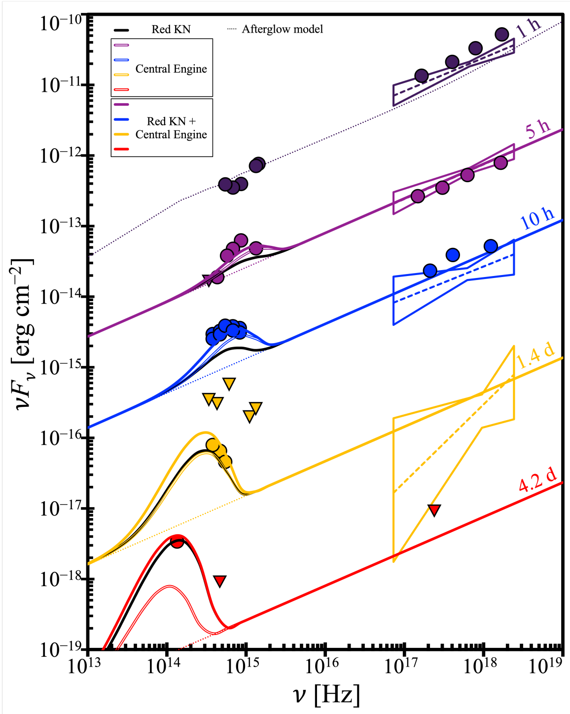
Figure 6. Same as Figure 3. The SED of our alternative central engine model where a low-power jet launched by late engine activity interacts with the lanthanide rich ejecta to explain the early (5 – 10 h) blue KN emission in GRB 211211A (double lines), while r-process explains the late (1.4 – 4.2 d) red KN emission (black line; same model as in Figures 2 and 3). The central engine model, combined with the red KN model (solid colored lines), can explain both early and late emission data [see Figure 6 for the bolometric luminosity].
